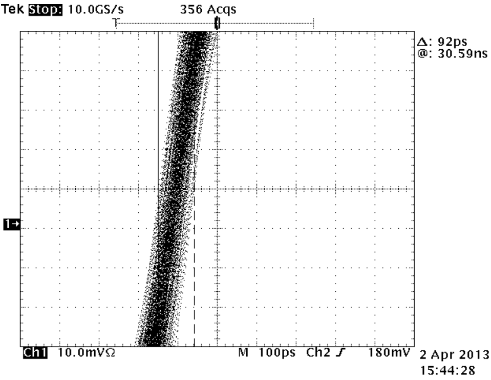
Illustration 6: Oscilloscope Trigger Jitter
