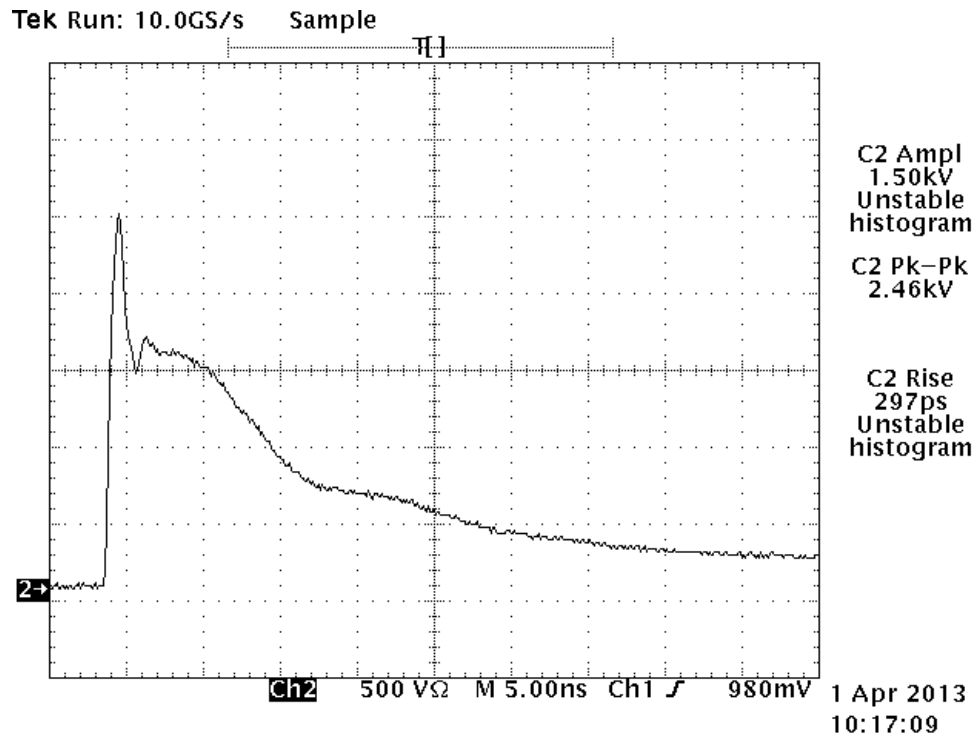
Illustration 1: Output Pulse Shape
