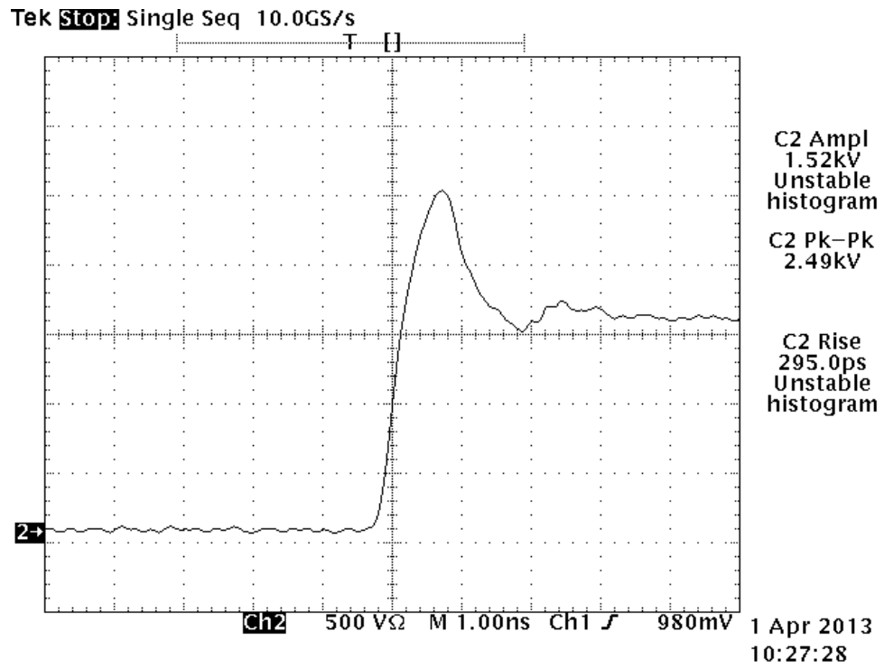
Illustration 2: Top Channel Risetime
