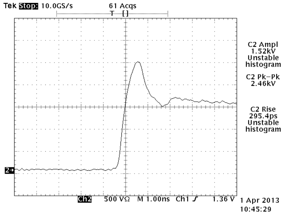
Illustration 3: Bottom Channel Risetime
