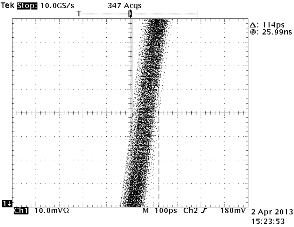
Illustration 5: Bottom Channel Jitter Including Oscilloscope Trigger Jitter
