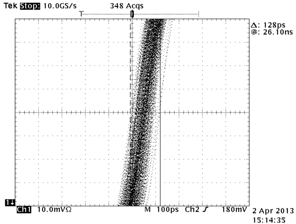
Illustration 4: Top Channel Jitter Including Oscilloscope Trigger Jitter
