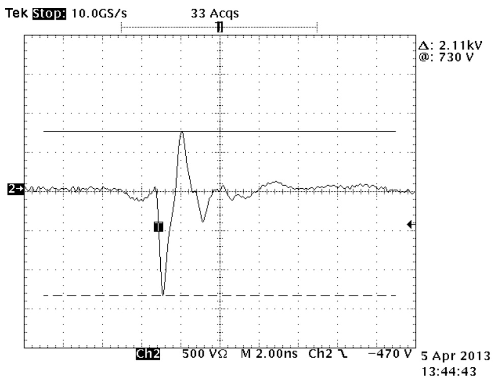
Illustration 1: Left Channel Output Pulse Shape
