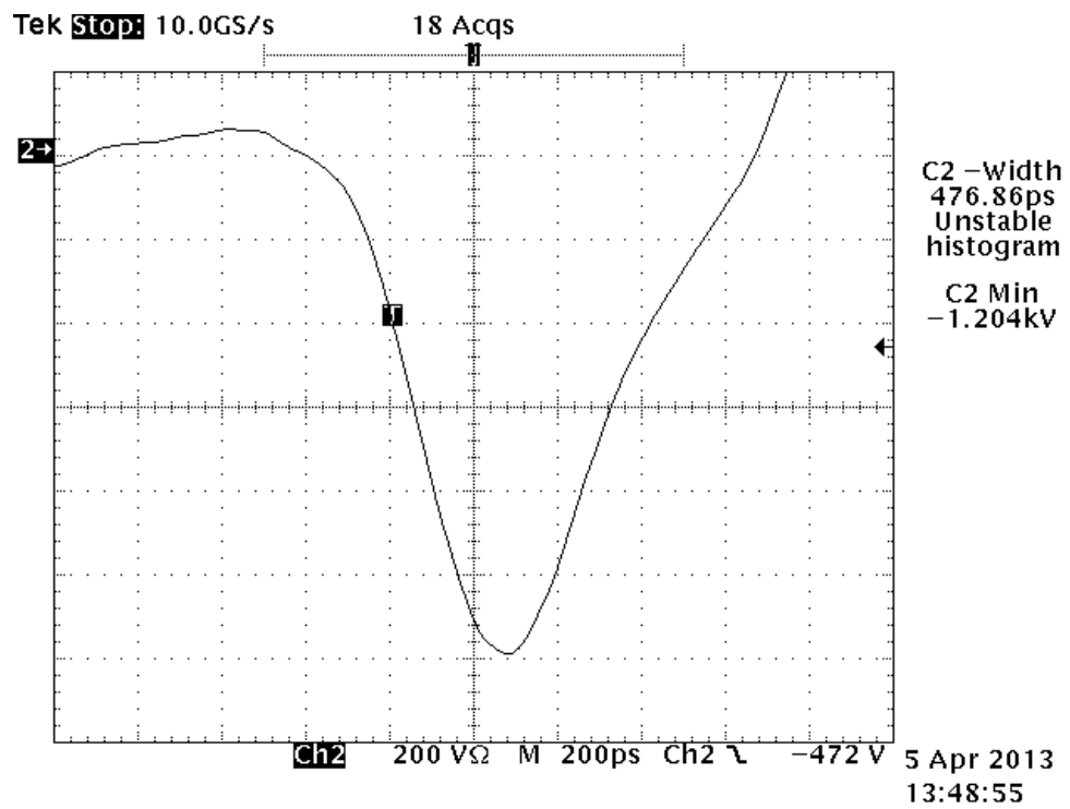
Illustration 4: Right Channel Negative Width
