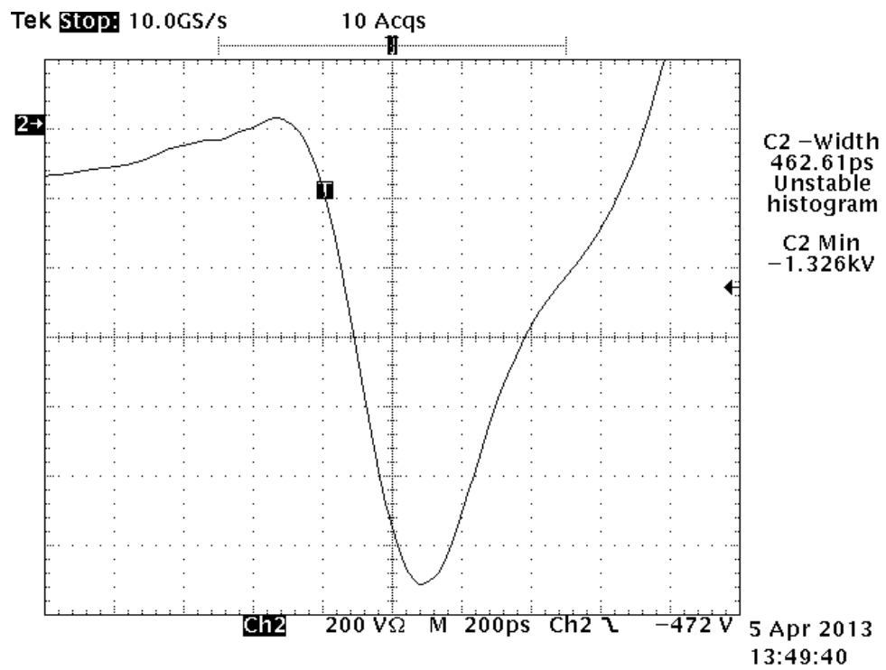
Illustration 3: Left Channel Negative Width
