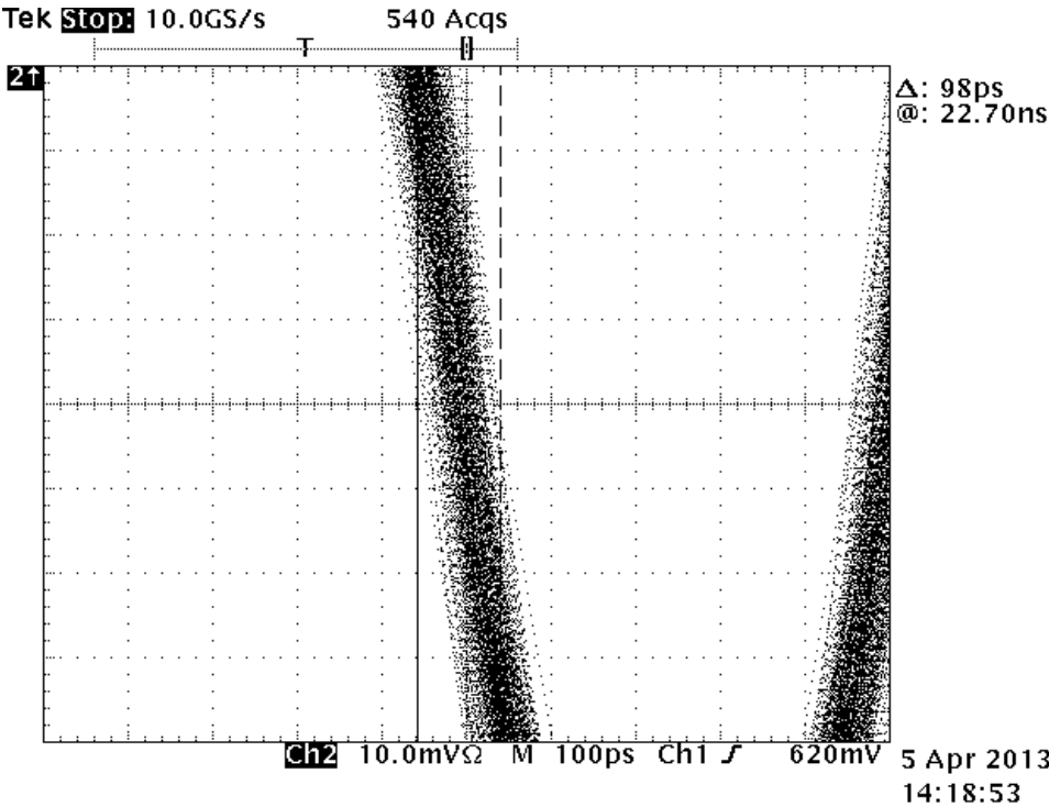
Illustration 6: Right Channel Jitter (Including Scope Trigger Jitter)
