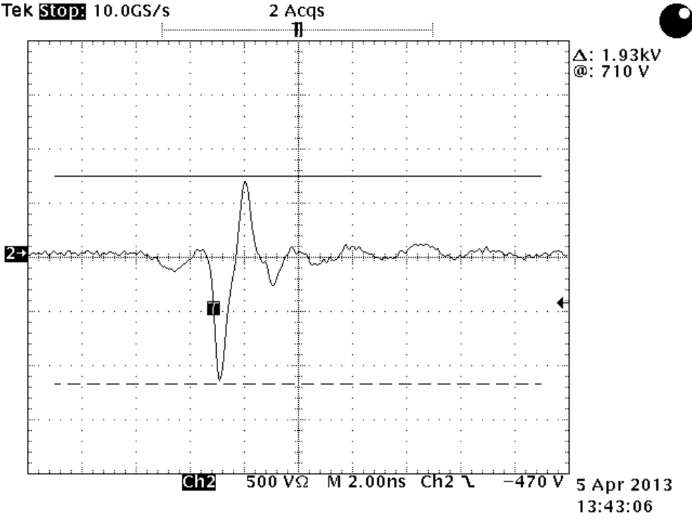
Illustration 2: Right Channel Output Pulse Shape
