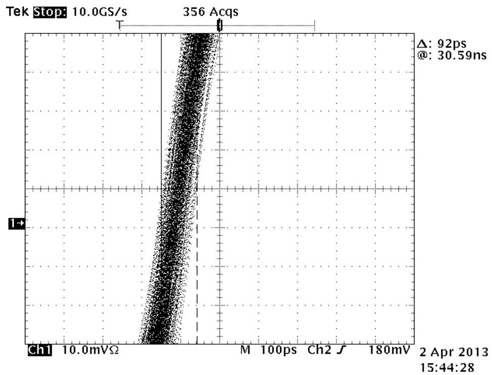
Illustration 7: Oscilloscope Trigger Jitter Including Voltage Noise
