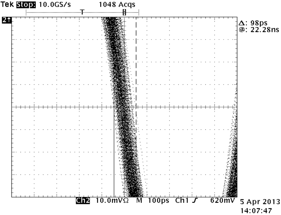
Illustration 5: Left Channel Jitter (Including Scope Trigger Jitter)
