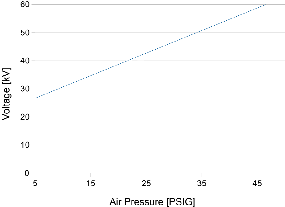
72850-502E Static Breakdown Voltage
